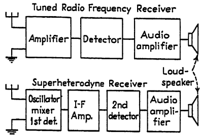
Detector positions in receivers.
